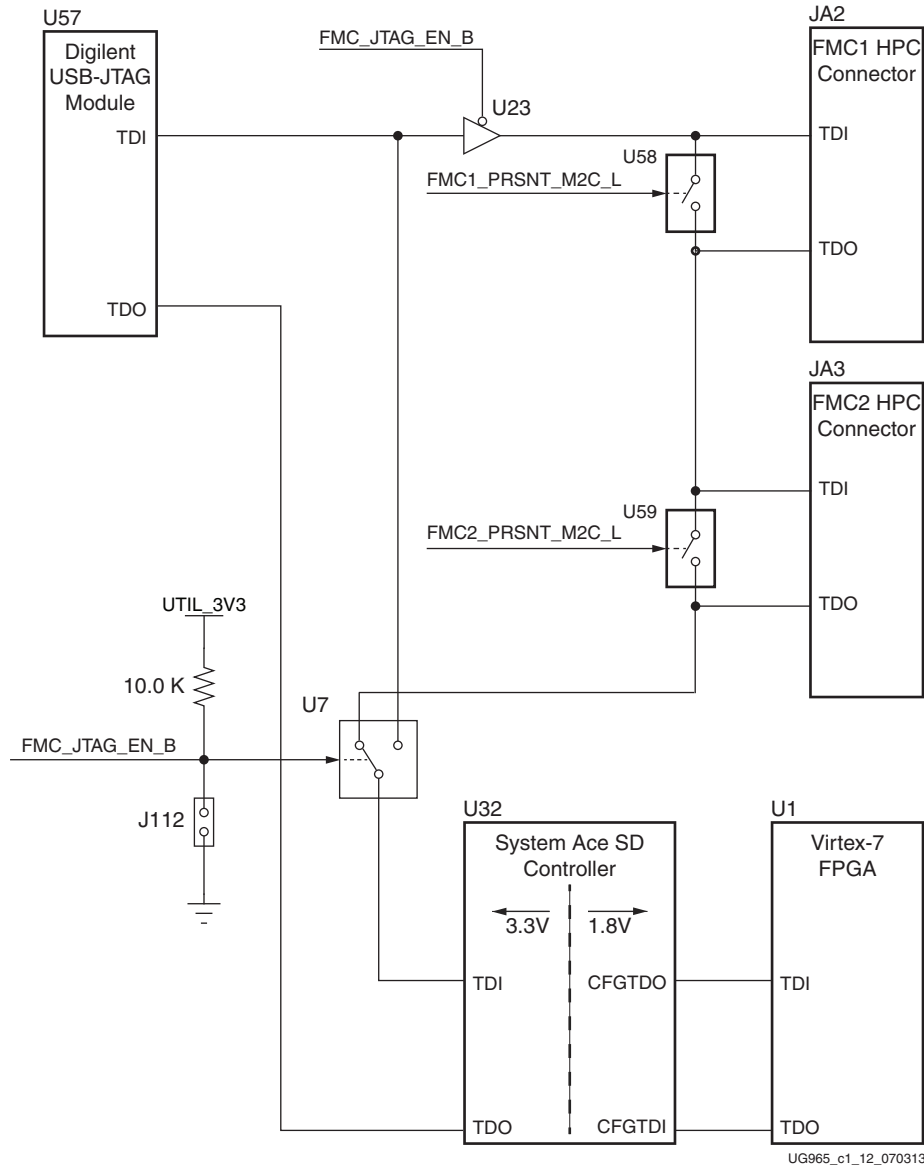
Figure 1-12: JTAG Chain
