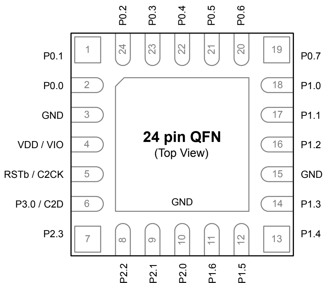
Figure 6.3. EFM8BB3x-QFN24 Pinout
