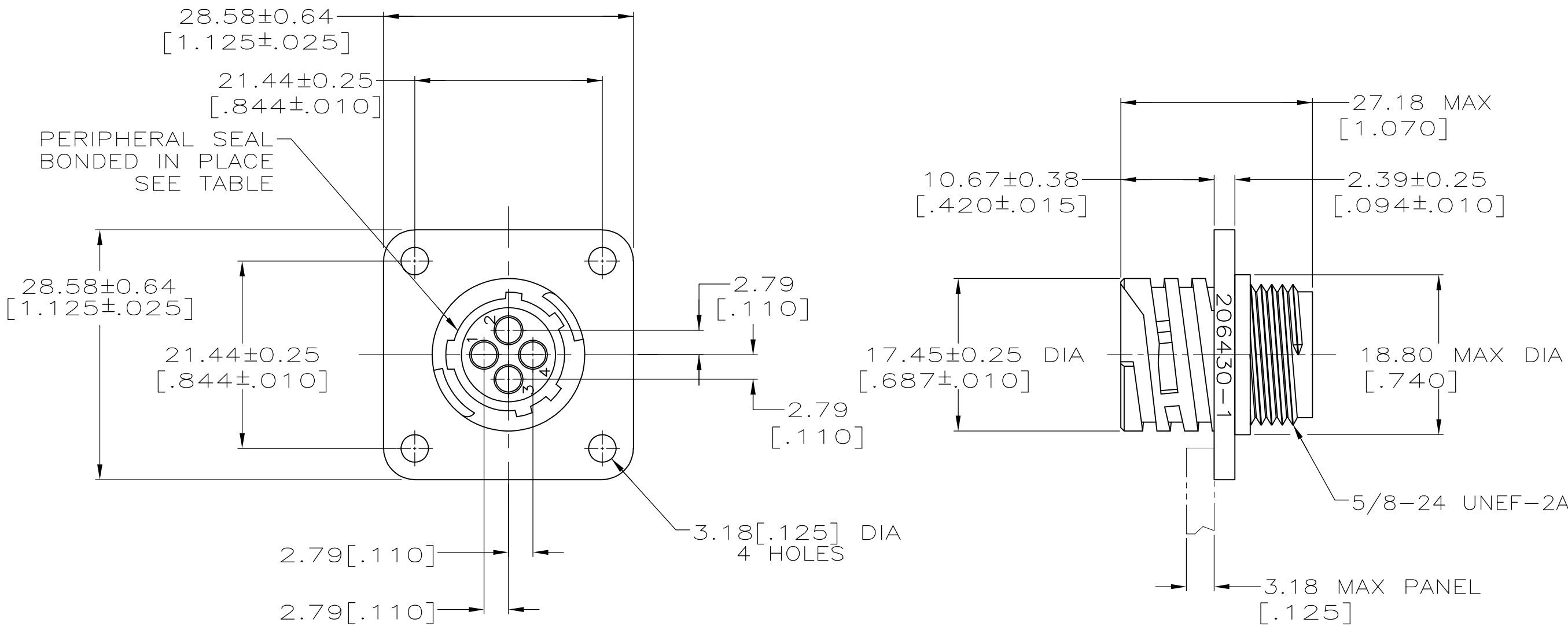
DETAIL A
