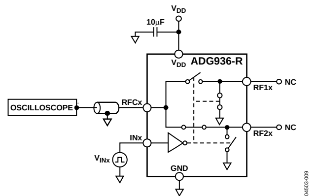
Figure 24. Video Feedthrough
