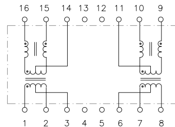
Circuit B
