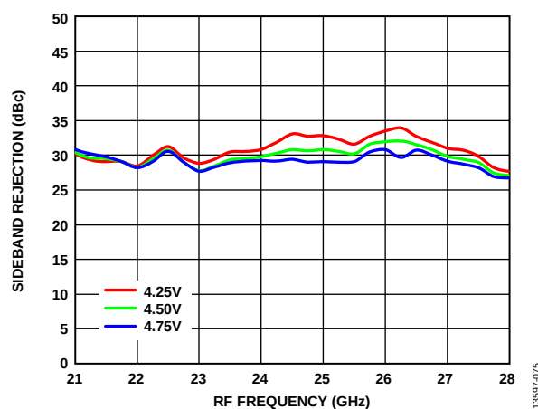
Figure 75. Sideband Rejection vs. RF Frequency over VDD1, LO Power = 4 dBm, T_A = 25^\circ\text{C}
