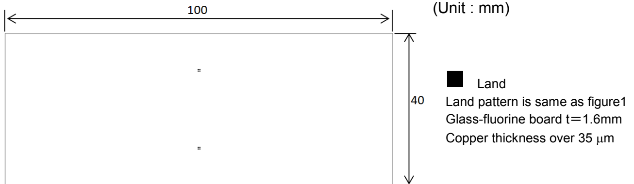
Fig. 2 Testing board
