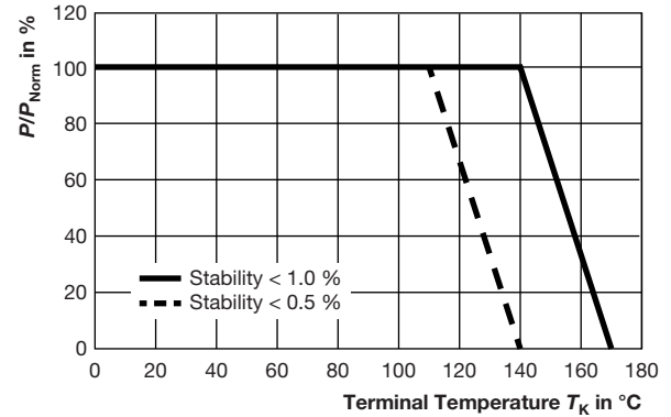
Fig. 2 - P_{100\text{ °C}} Rated Power; of Standard Electrical Specification Table Example L5000
