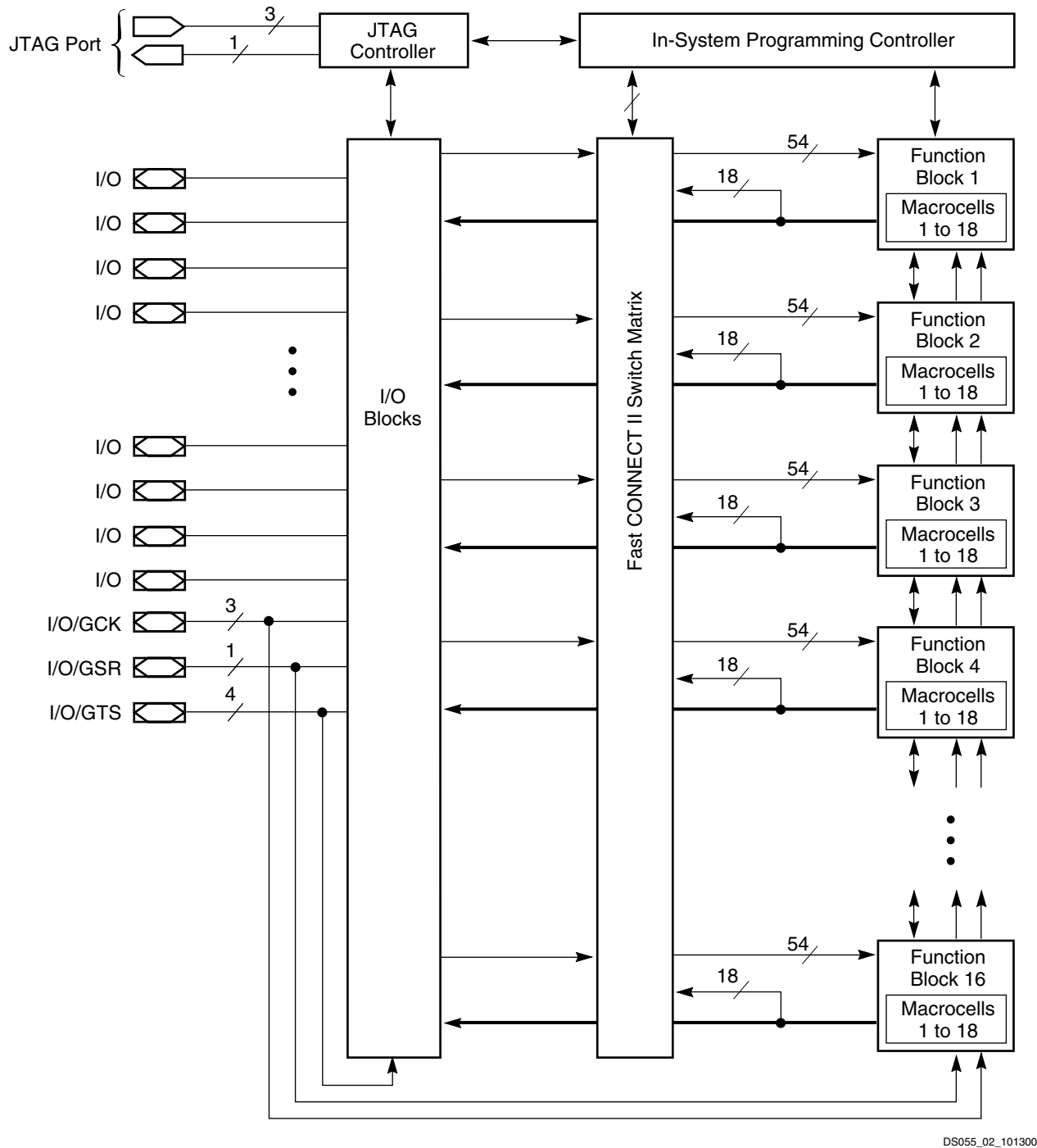
Figure 2: XC95288XL Architecture
