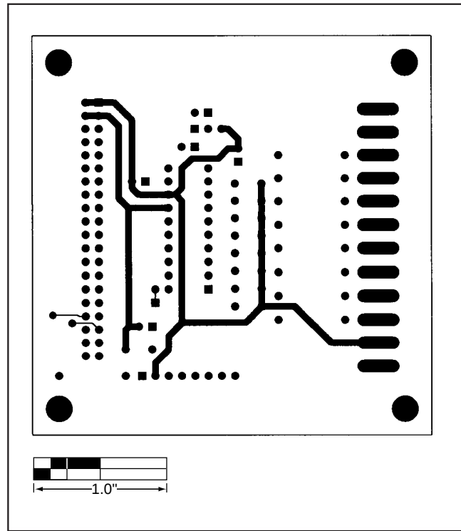
Figure 3. MAX1110 EV Kit PC Board Layout—Component Side
