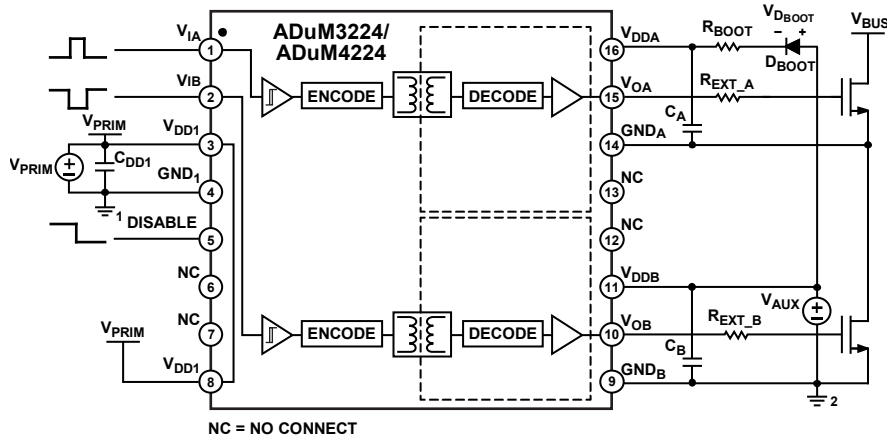
NC = NO CONNECT 1 GND 1 IS CONNECTED TO THE PRIMARY SIDE GROUND, ISOLATED FROM THE SECONDARY GROUND. 2 GND 2 IS CONNECTED TO THE SECONDARY SIDE GROUND, ISOLATED FROM THE PRIMARY GROUND.
