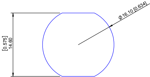
PANEL CUTOUT
