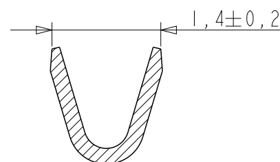
SECTION B - B SCALE 15/1
