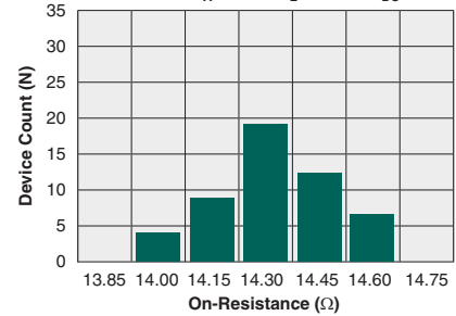
Typical On-Resistance Distribution (N=50, T_A=25^\circ\text{C} , I_L=120\text{mA}_{\text{DC}} )
