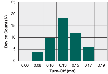
Typical Turn-Off Time (N=50, T_A=25^\circ\text{C} , I_L=120\text{mA}_{\text{DC}} , I_F=5\text{mA} )
