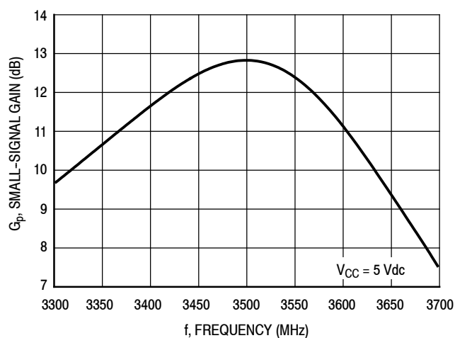
Figure 46. Small-Signal Gain (S21) versus Frequency
