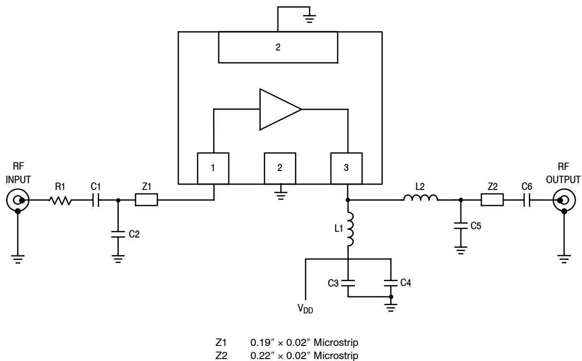
Figure 3. MMG30301BT1 Test Circuit Schematic
