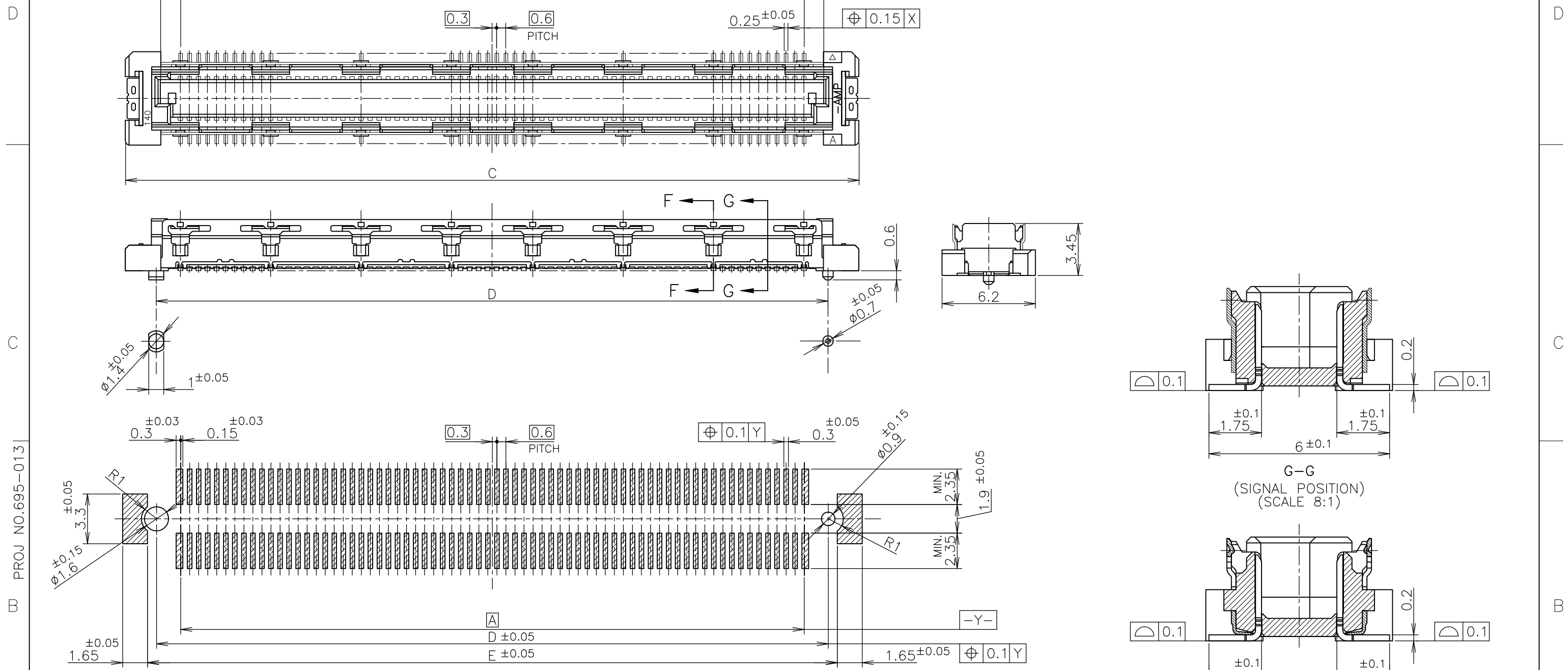
REFERENCE P.C.BOARD LAYOUT G-G (SIGNAL POSITION) (SCALE 8:1) F-F (GROUND POSITION) (SCALE 8:1)
