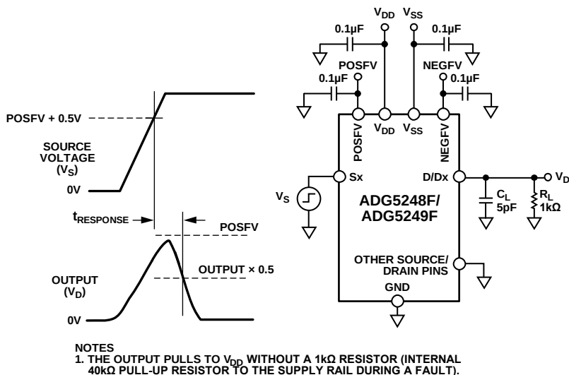
Figure 43. Overtolerance Response Time, t_{RESPONSE}
