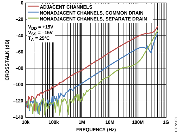
Figure 23. Crosstalk vs. Frequency, \pm 15 V Dual Supply
