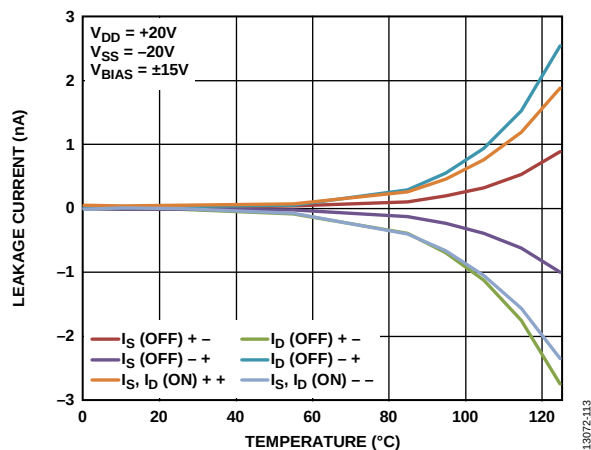
Figure 15. Leakage Current vs. Temperature, \pm 20V Dual Supply
