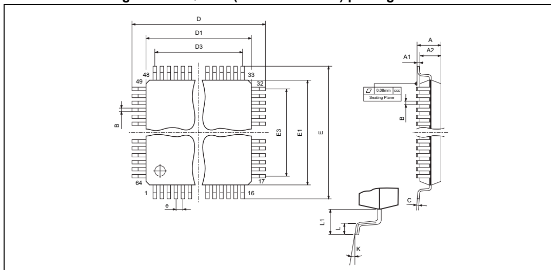
Figure 11. TQFP64 (10 mm x 10 mm) package outline
