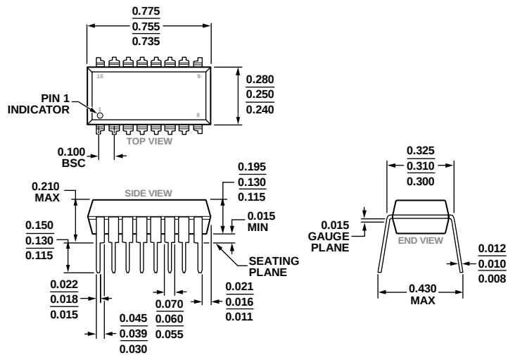
Figure 22. 16-Lead Plastic Dual In-Line Package [PDIP]
