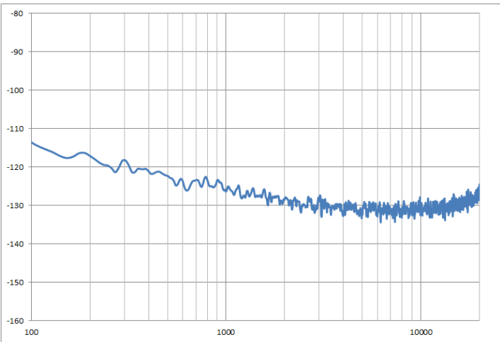
Figure 6: Noise Level
