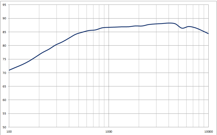
Figure 5: Typical PSRR
