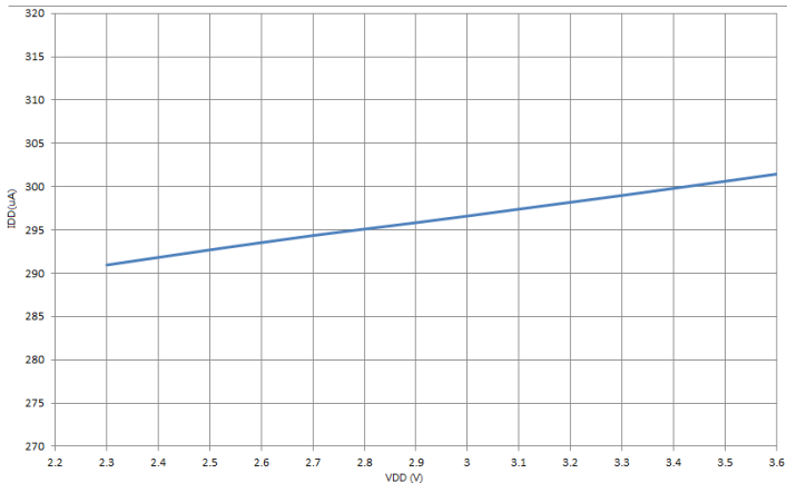
Figure 6: Typical Idd vs Vdd
