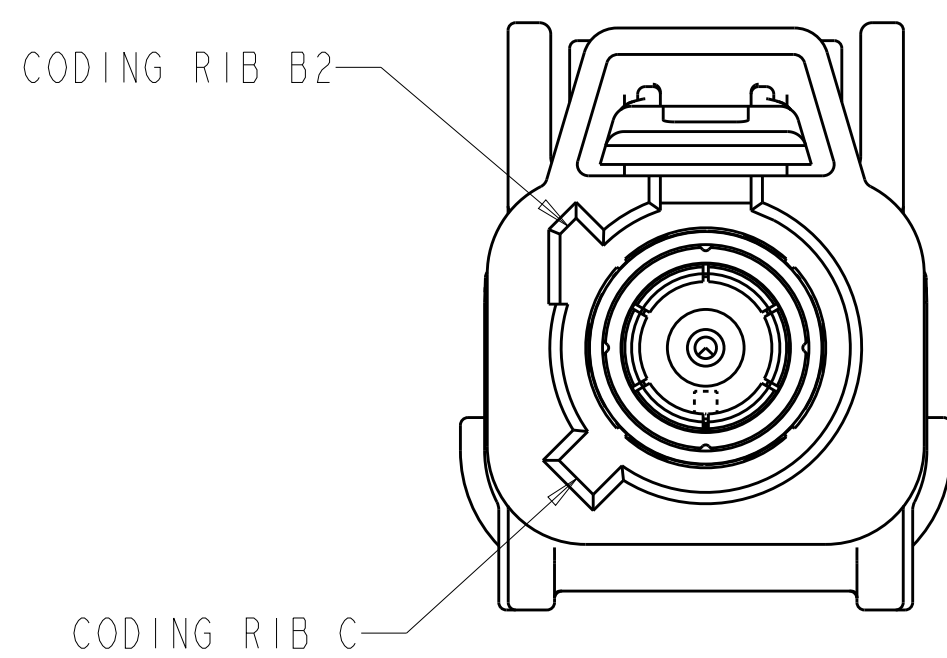
DETAIL H
