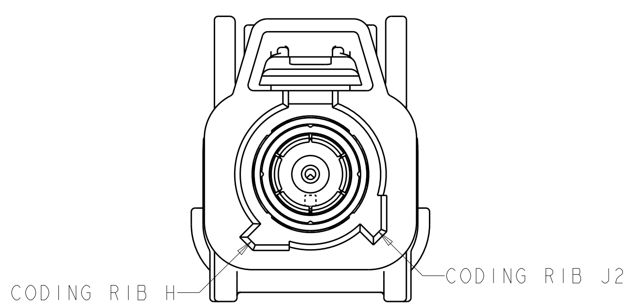
DETAIL M
