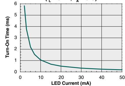
Typical Turn-On Time vs. LED Forward Current (I L =75mA, T A =25°C)
