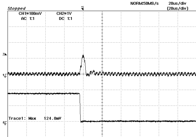
Figure 21: Typical transient response to step load change at 2.5\text{A}/\mu\text{S} from 100% to 50% of I_o , max at 5\text{V}_{in} , 1.8\text{V}_{out} ( C_{out} = 1\mu\text{F} ceramic, 10\mu\text{F} tantalum)
