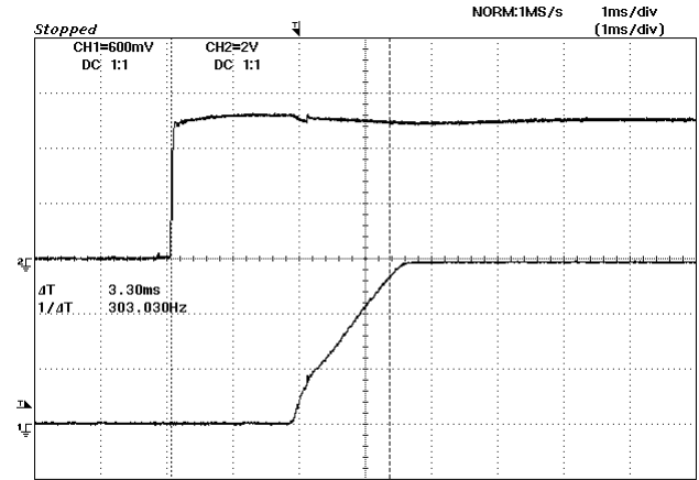
Figure 14: Turn on delay time at 5Vin, 1.8V/6A out
