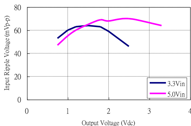
Figure 33: Input voltage ripple for various output models, I_o = 6A ( C_{IN} = 4 \times 100\mu F tantalum // 2 \times 47\mu F ceramic)
