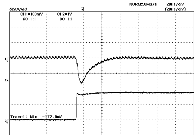
Figure 24: Typical transient response to step load change at 2.5A/μS from 50% to 100% of I_o , max at 3.3Vin, 2.5Vout (Cout = 1μF ceramic, 10μF tantalum)
