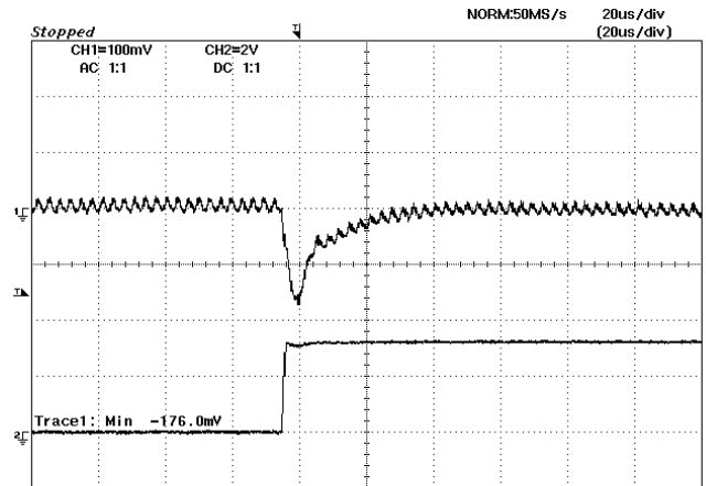
Figure 20: Typical transient response to step load change at 2.5\text{A}/\mu\text{S} from 50% to 100% of I_o , max at 5\text{V}_{in} , 3.3\text{V}_{out} ( C_{out} = 1\mu\text{F} ceramic, 10\mu\text{F} tantalum)
