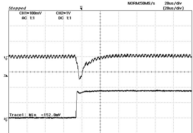
Figure 22: Typical transient response to step load change at 2.5\text{A}/\mu\text{S} from 50% to 100% of I_o , max at 5\text{V}_{in} , 1.8\text{V}_{out} ( C_{out} = 1\mu\text{F} ceramic, 10\mu\text{F} tantalum)
