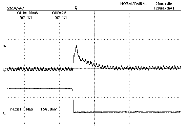
Figure 19: Typical transient response to step load change at 2.5\text{A}/\mu\text{S} from 100% to 50% of I_o , max at 5\text{V}_{in} , 3.3\text{V}_{out} ( C_{out} = 1\mu\text{F} ceramic, 10\mu\text{F} tantalum)
