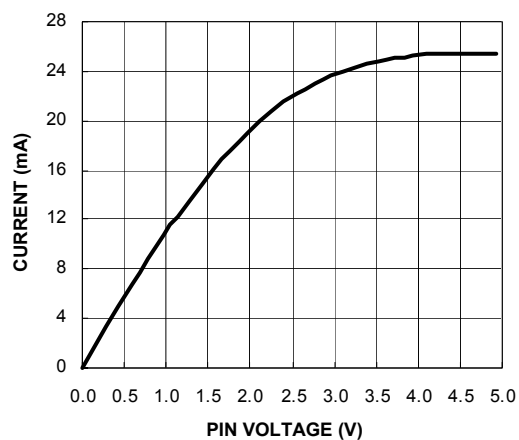
FIGURE 15. STATUS/FAULT PIN VOLTAGE vs CURRENT WHEN THE OPEN-DRIVE MOSFET TURNS ON
