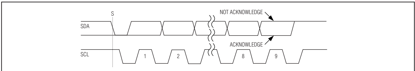
Figure 6. Acknowledge Bits
