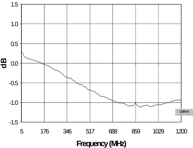
Insertion Loss Pin 4-3
