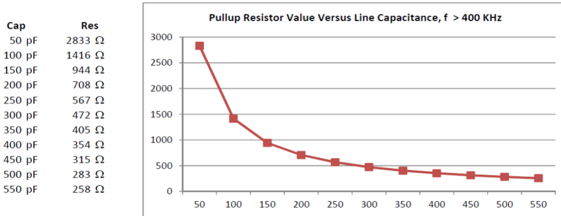
Figure 19. Pull-up Resistor Value
