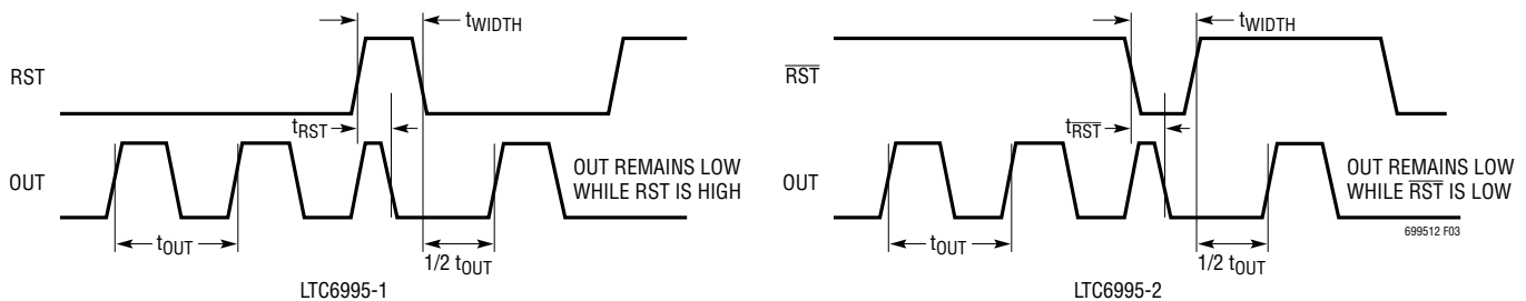
Figure 3. Reset Timing Diagram (POL Bit = 0)
