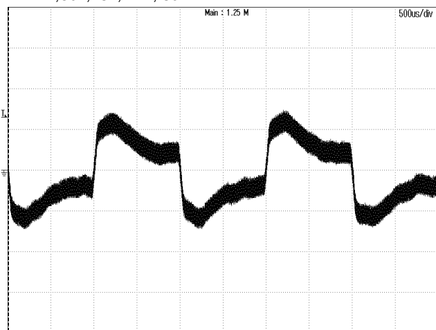
Figure 3: Dynamic response to load step 11A~16.5A with 0.1A/uS slew rate at 48Vin CH1:VOUT, 100mV/div, 500uS/div
