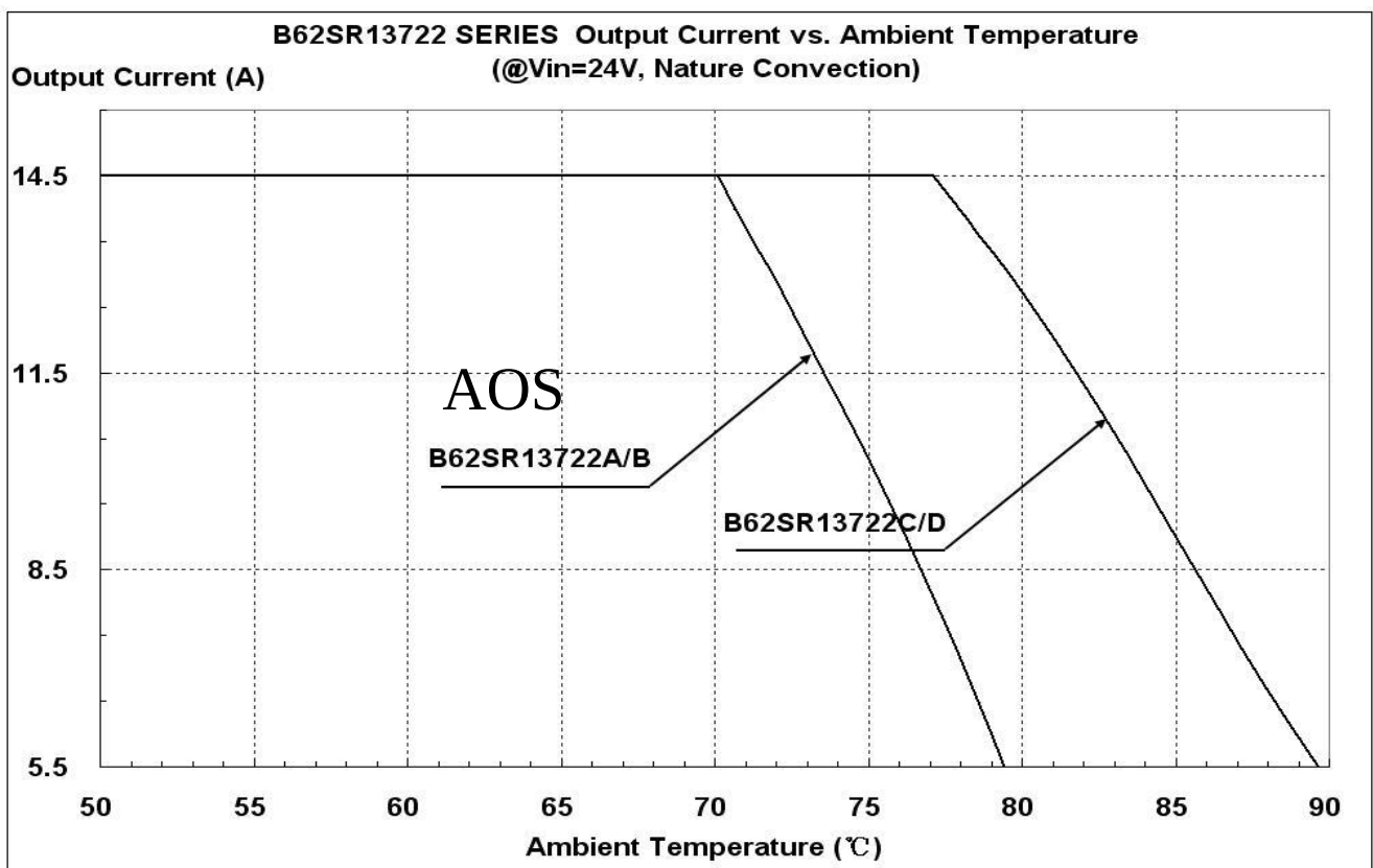
Figure 17: Output Current vs. Ambient temperature @ Vin=24V
