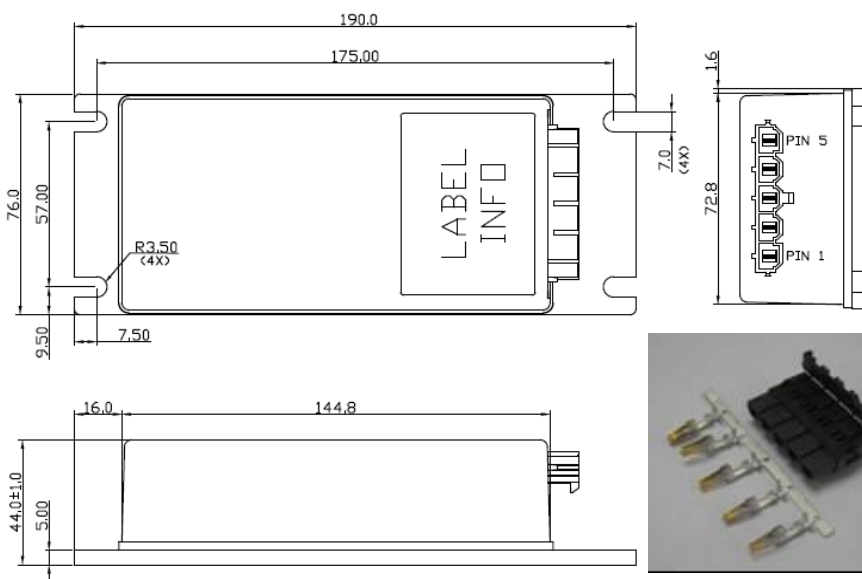
B62SR13722CC
