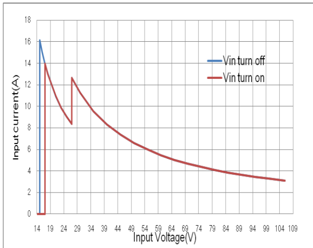
Figure 7: Input current vs. Input voltage @ Vin=18V~27V, 200W; Vin=27V~106V, 300W
