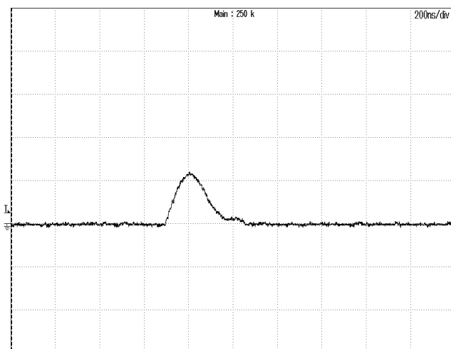
Figure 11: Inrush current @ Vin=48V CH1:lin, 2A/div, 200nS/div; Max current 2.4A, I_{2t}=1.24E-7 A^2S
