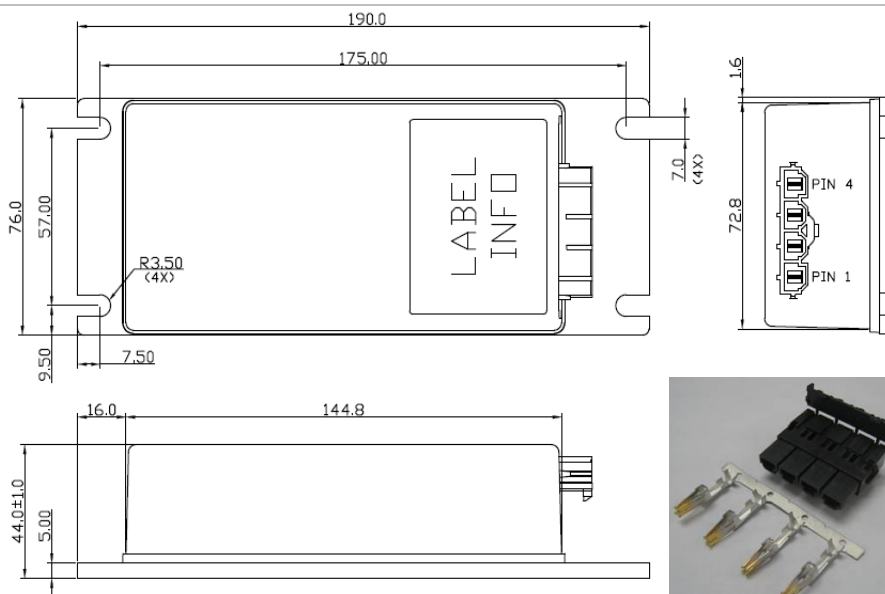
B62SR13722DC
