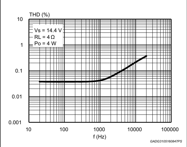
Figure 12. Distortion vs. frequency (4 \Omega )
