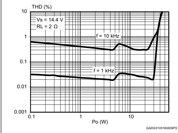
Figure 11. Distortion vs. output power (2 \Omega , SBI mode)
