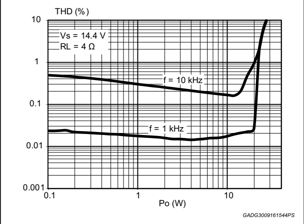
Figure 8. Distortion vs. output power (4 \Omega , STD mode)
