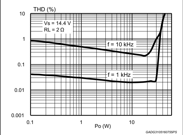
Figure 10. Distortion vs. output power (2 \Omega , STD mode)
