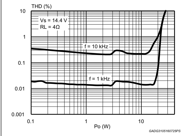
Figure 9. Distortion vs. output power (4 \Omega , SBI mode)
