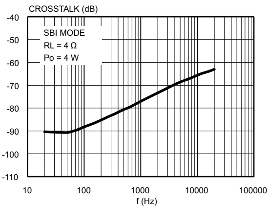
Figure 23. Crosstalk vs. frequency (SBI mode)
