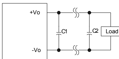
Figure 17 Output ripple filter for a distant load
