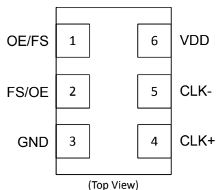
Pin Assignments
