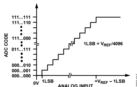
Figure 34. Transfer Characteristic
