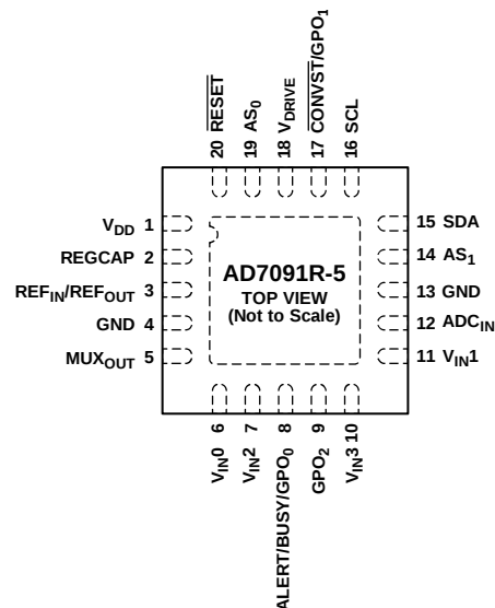
Figure 4. Pin Configuration, 20-Lead LFCSP
