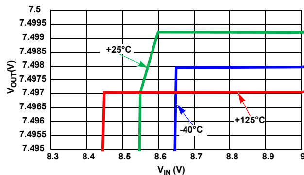
FIGURE 67. DROPOUT WITH -10\text{mA} LOAD
