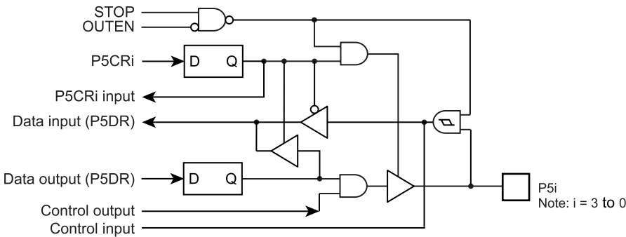
Figure 5-7 Port P5
