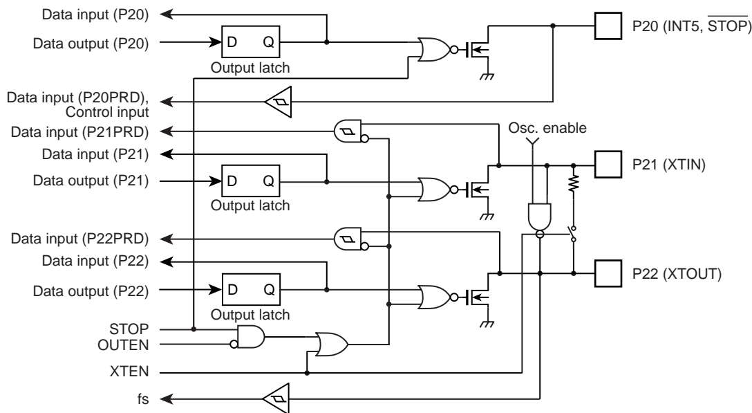
Figure 5-4 Port P2
