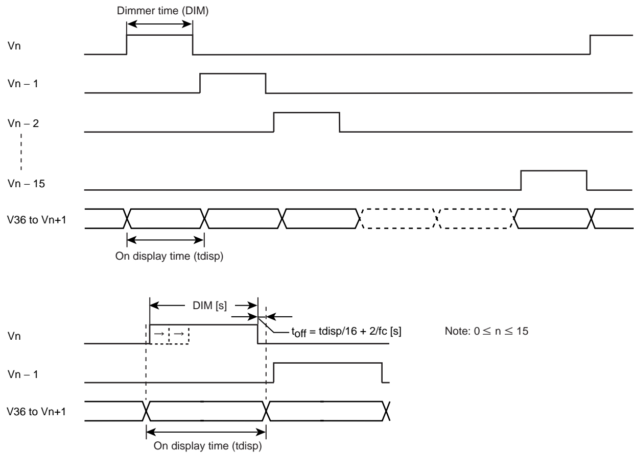
Figure 15-3 VFT Drive Wafeform and Display Timing
