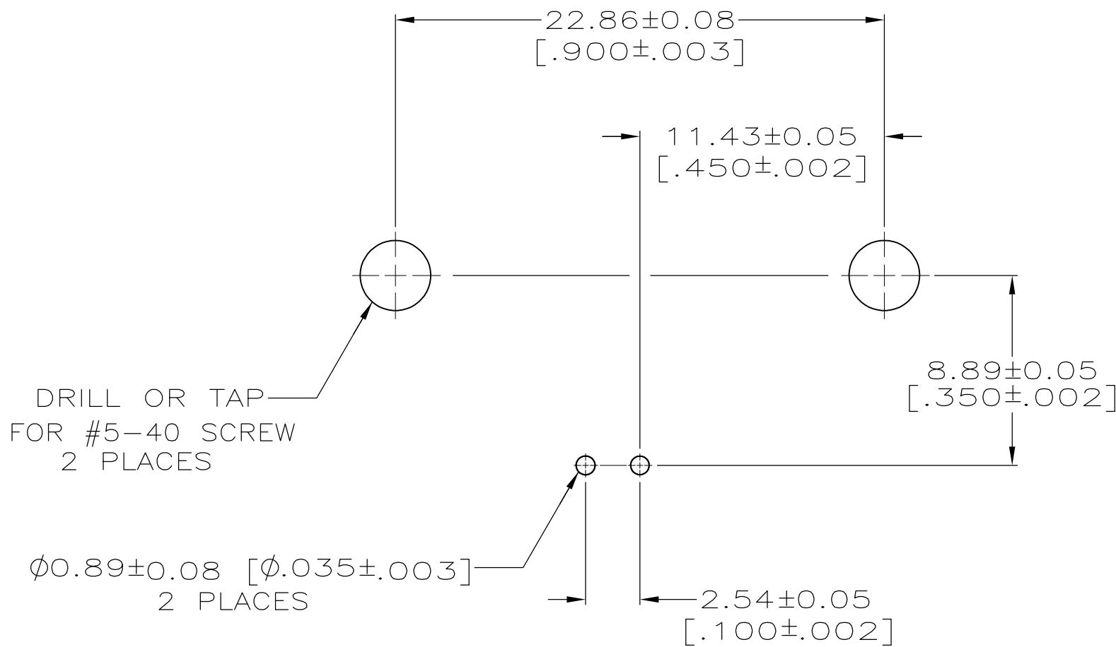
PCB CONFIGURATION
