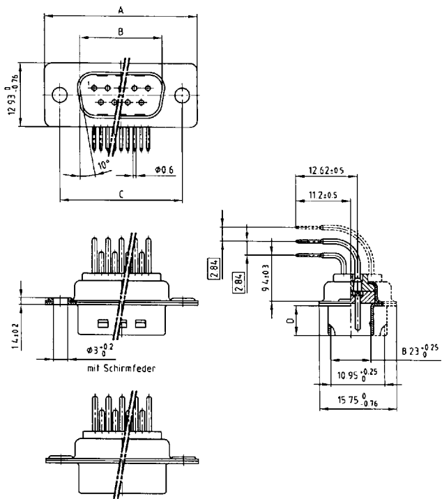
Plug connector
