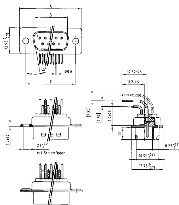
Plug connector
