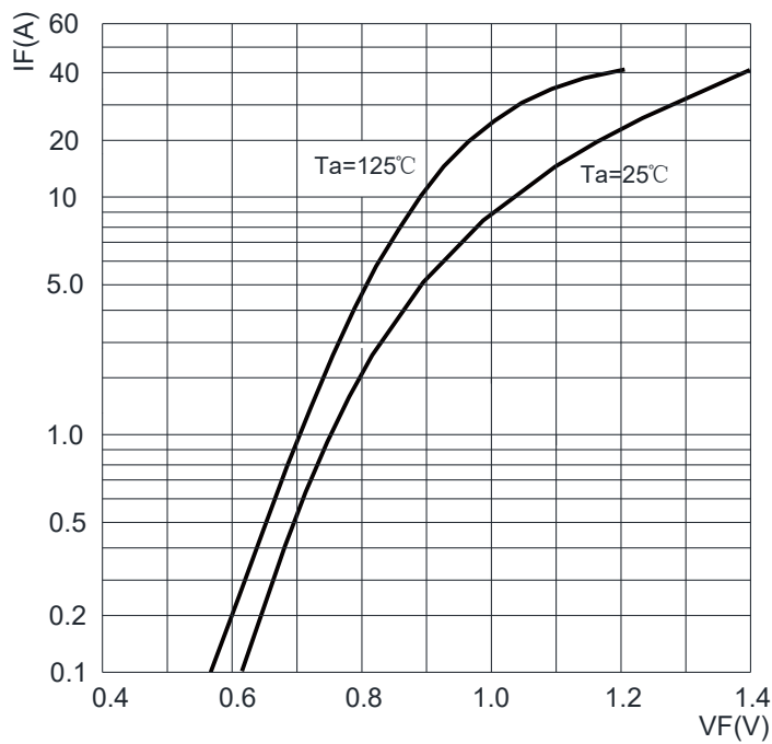
FIG3: Forward Voltage
