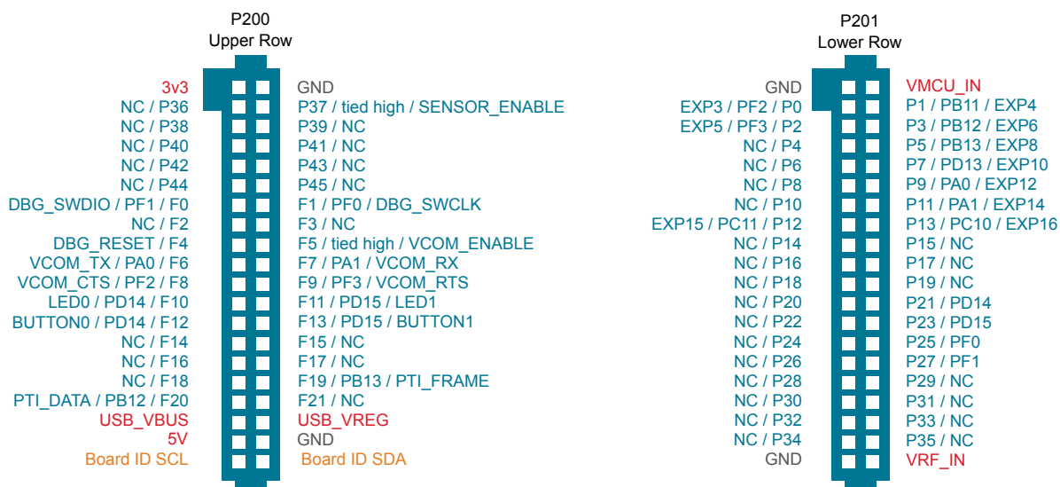
Figure 3.1 Radio Board Connectors
