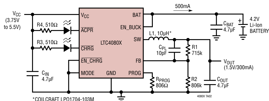
Li-Ion Battery Charger with 1.5V Buck Regulator
