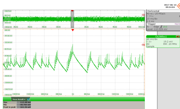
Figure 54 – 265 VAC Input.
