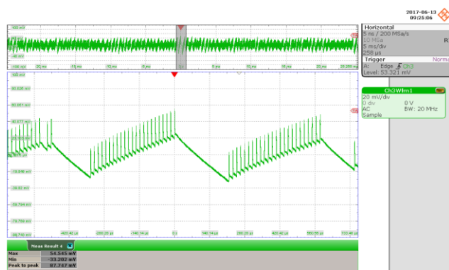
Figure 53 – 85 VAC Input.
