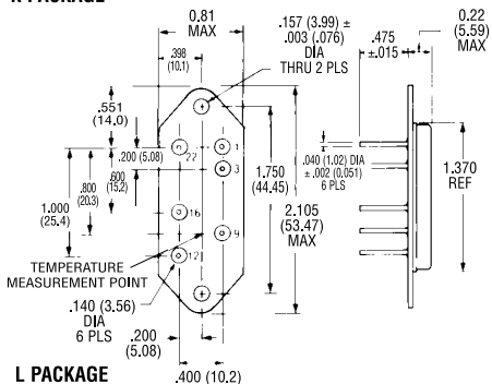
L PACKAGE
