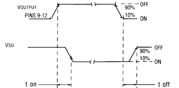
STATUS TURN-ON AND TURN-OFF TIMING FIGURE 6
