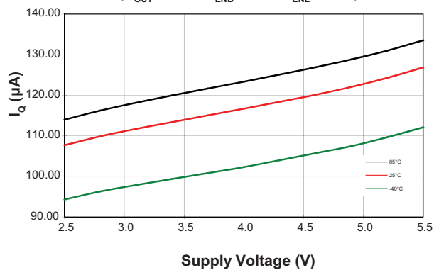
Buck Quiescent Current vs Supply Voltage (V_{OUT} = 1.2V, V_{ENB} > 1.5V, V_{ENL} < 0.4V)
