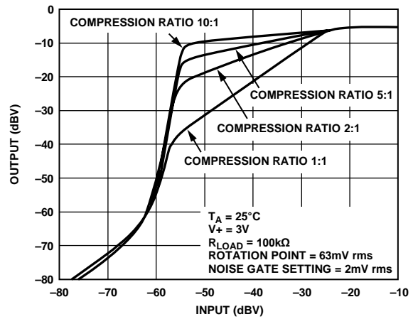
Figure 7. Output vs. Input Characteristics
