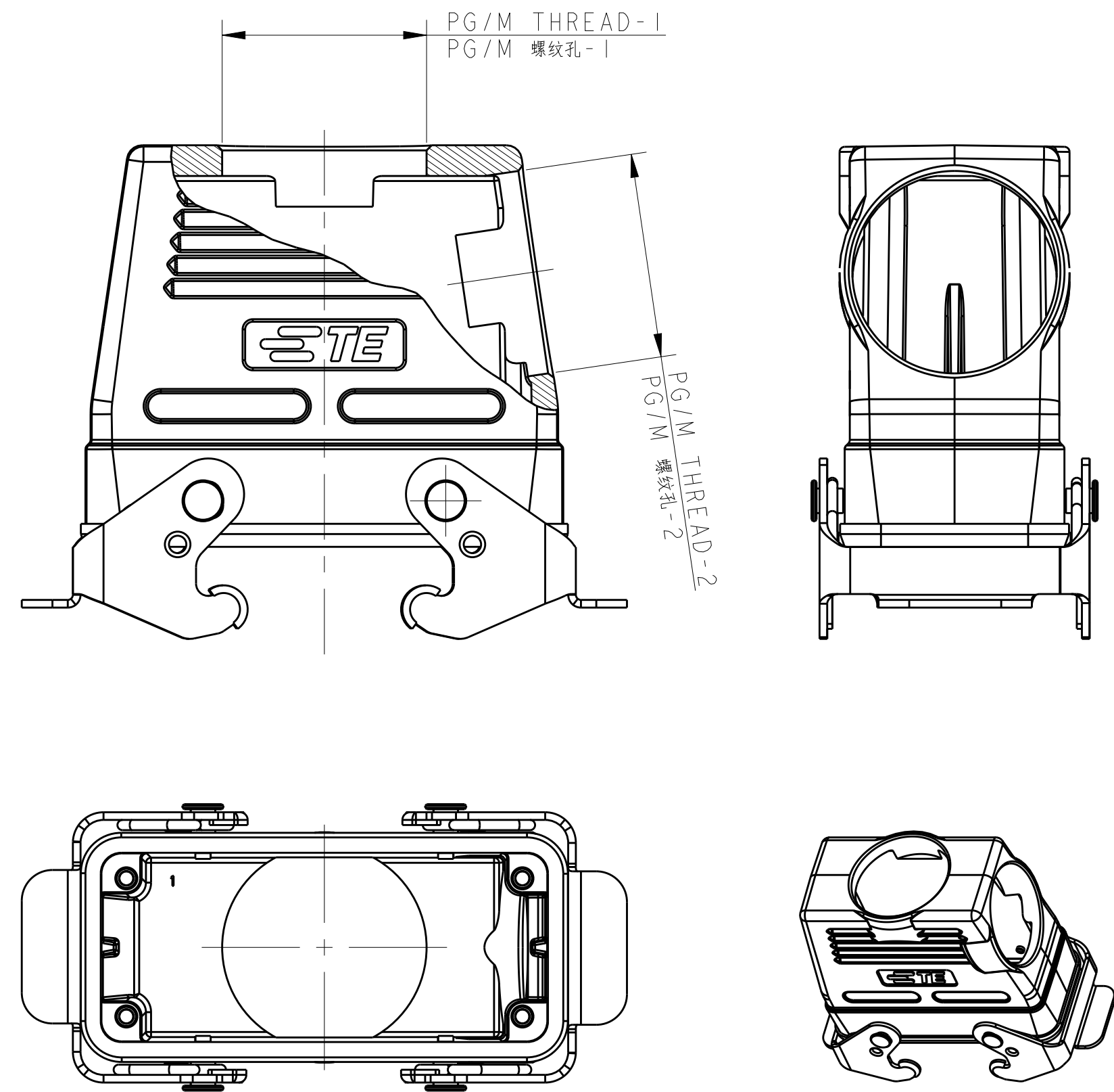
TYPE 8: HIGH CONSTRUCTION + METAL DOUBLE LOCKING 2 ENTRY HOLE
