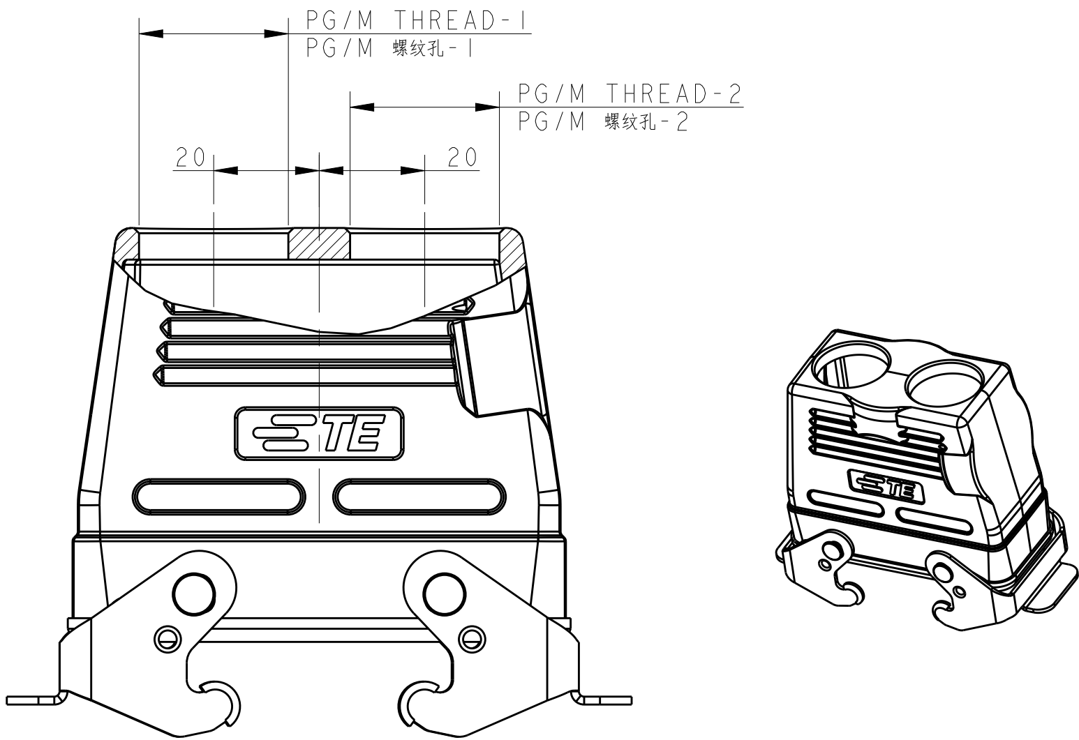
TYPE 7: HIGH CONSTRUCTION + METAL DOUBLE LOCKING 2 ENTRY HOLE
